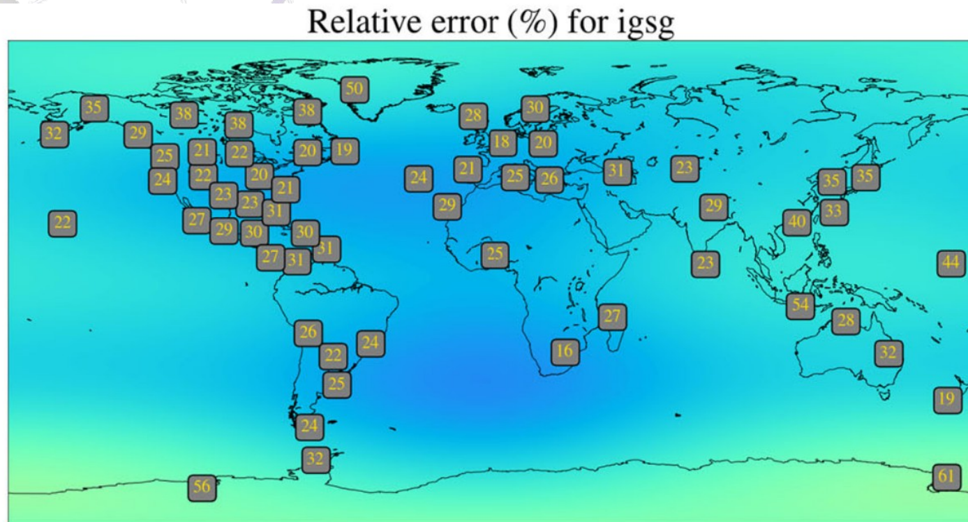
Fig. 8 Map approximating the spatial distribution of dSTEC relative error for classical IGS GIMs (left hand column, for IGSG,
