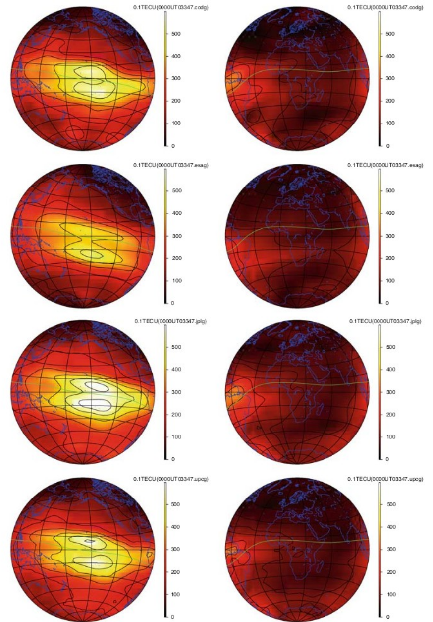
Fig. 4 Example of IAAC VTEC maps snapshots, for day 347 (13 Dec) of 2003, at 00UT. Every row, from top to bottom, corresponds to CODE, ESA, JPL and UPC. The units for all maps are tenths of a TECU
