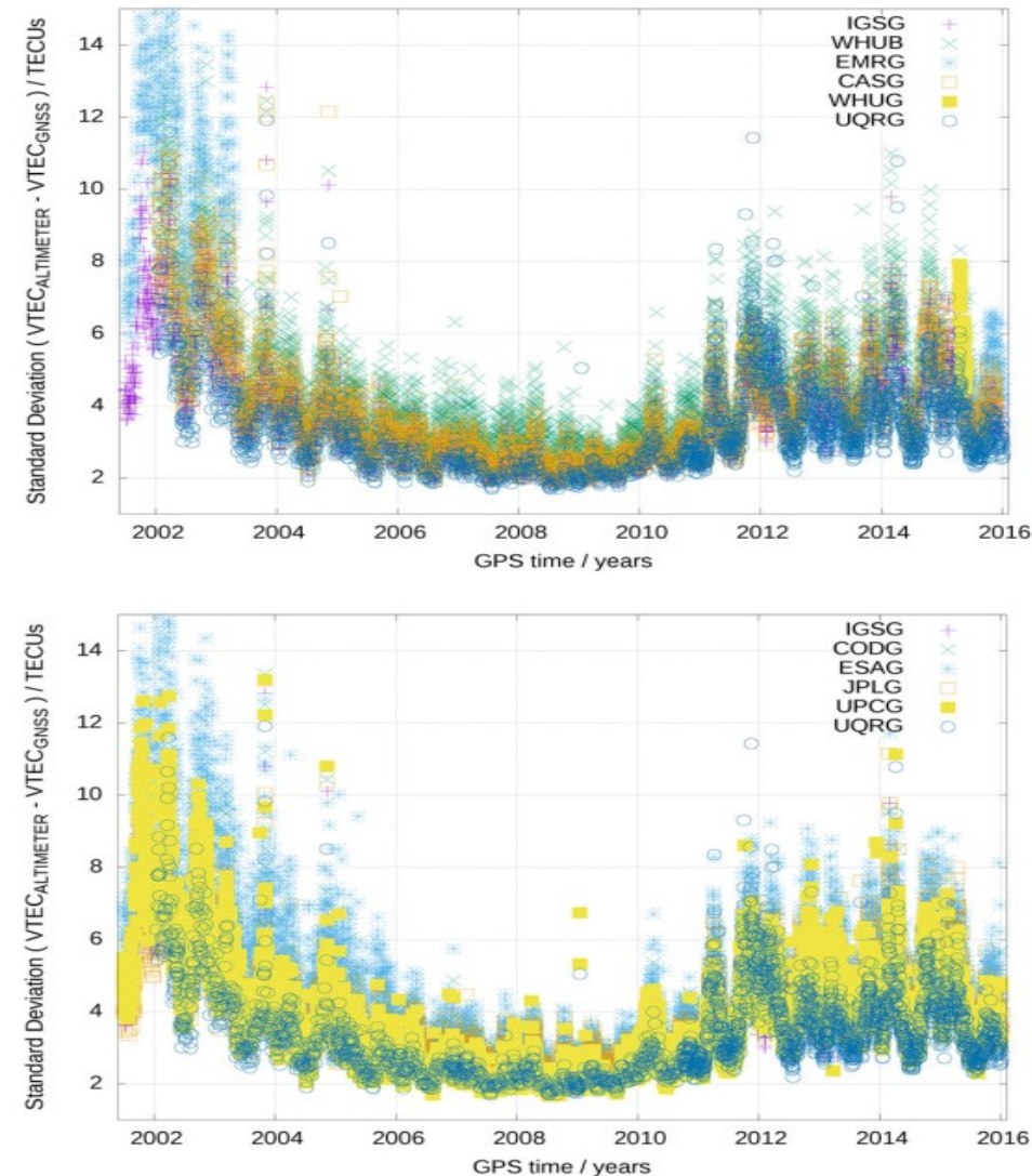
Fig. 3 Daily standard deviation of the VTEC difference regarding altimeter VTEC measurements, involving new GIMs (top plot) and classical GIMs (bottom plot). The comparison has been performed over the same dataset referenced in Fig. 1
