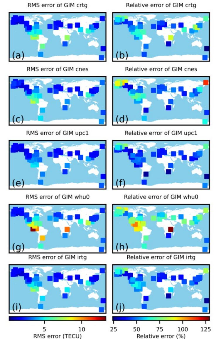
Figure 4. The distribution of dSTEC-GPS results on 5 January 2021 (after the improvement of the UPC interpolation technique).
